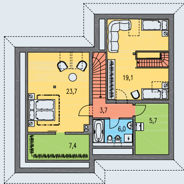
POSCHODIE [plocha 65.7 m 2 ]
