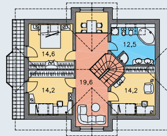
POSCHODIE [plocha 83.4 m 2 ]
