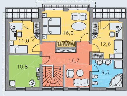
POSCHODIE [plocha 85.0 m 2 ]
