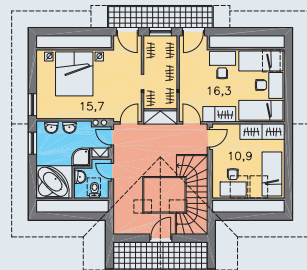
POSCHODIE [plocha 93.6 m 2 ]
