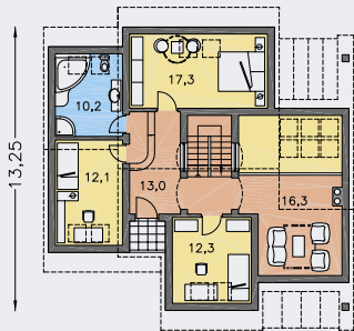
POSCHODIE [plocha 82.6 m 2 ]
